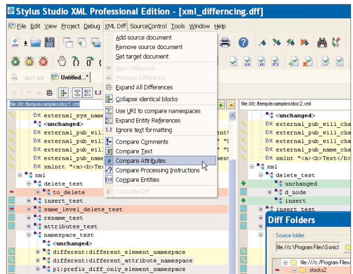
Visually compare XML files and folders with Stylus Studio.
