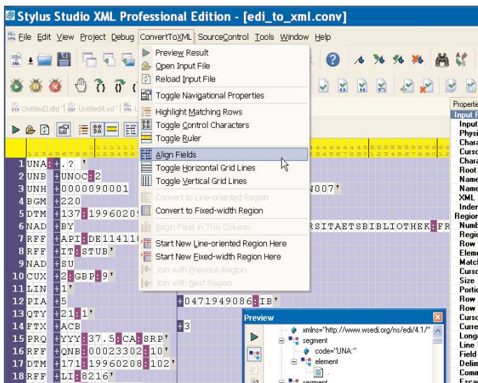
Visually convert an EDI file to an XML data format.
