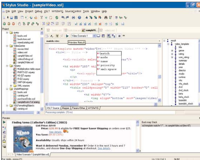
The XSLT editor has built-in Sense:Xtm intelligent XML editing including context-sensitive knowledge of all XSLT instructions and XPath functions to ensure syntactically correct XSLT stylesheets.
